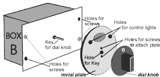
B) Control box for interior mounting (invisible box -> see separate installation sheet)
