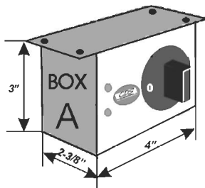
A) Control box for under counter/table mounting (visible box)
